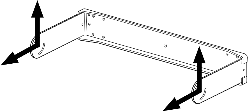
ArenaMatch Full-Range DeltaQ Array AMUBRKT - U-bracket for use with AM10, AM20, AM40 WLL = one AM module (40 kg [85 lbs])
