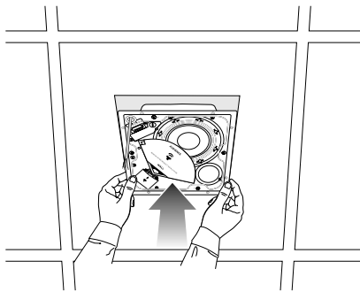
Fig. 1. Install loudspeaker.
