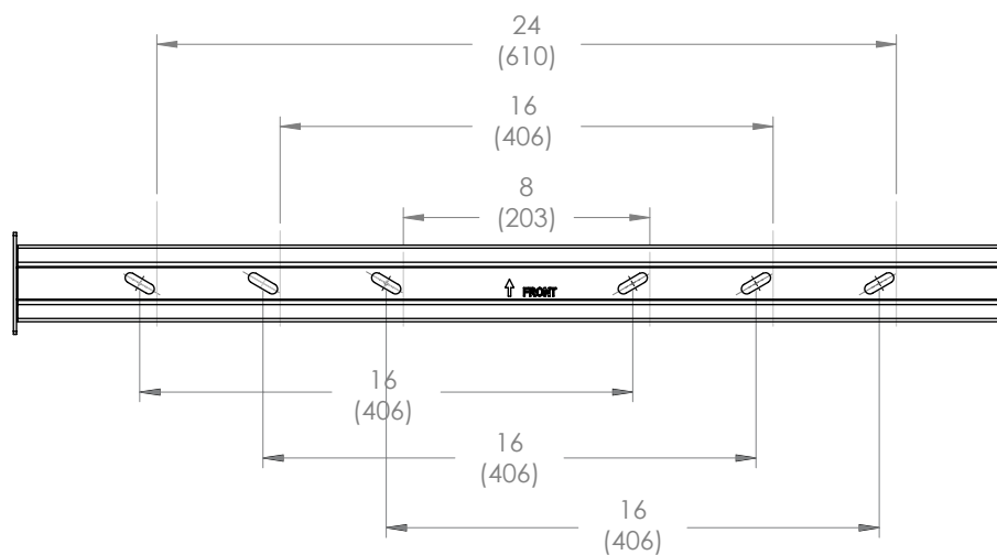
WALL PLATE MOUNTING HOLES
